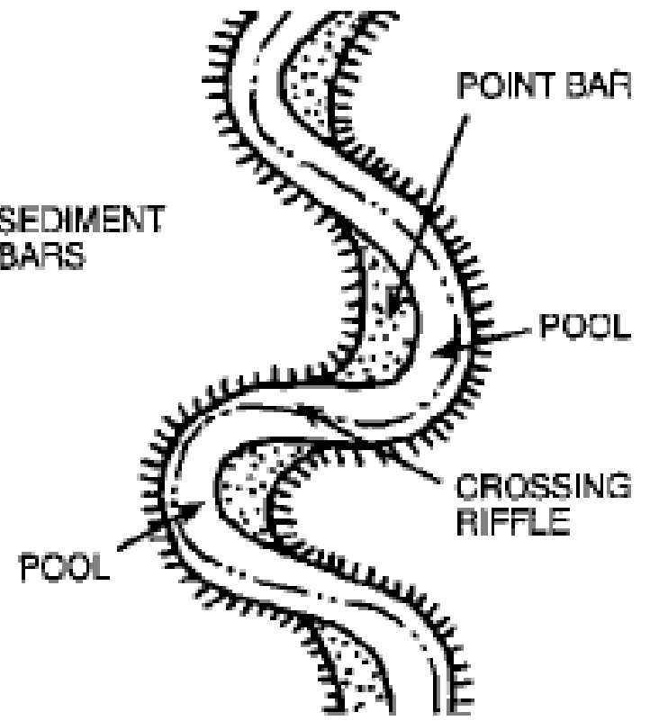
MEANDERING CHANNEL SINUOSITY >1.5
